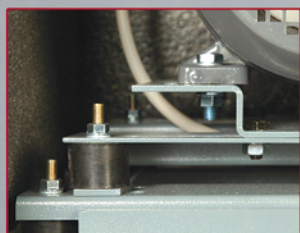
STRUCTURE WITH VIBRATION DAMPERS Double anti-vibration support to eliminate vibration and reduce the level of noise.
