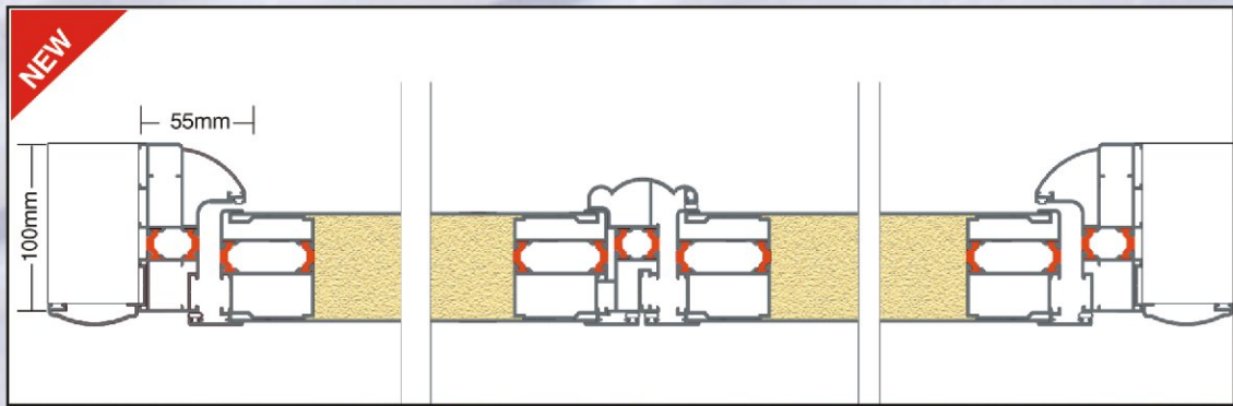
New Thermo break system with 16mm polyamide which ensures heat insulation.
