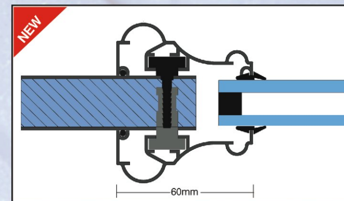
Clip Lock System
